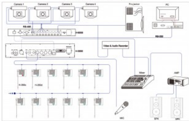
H-3000 System Connection Diagram
