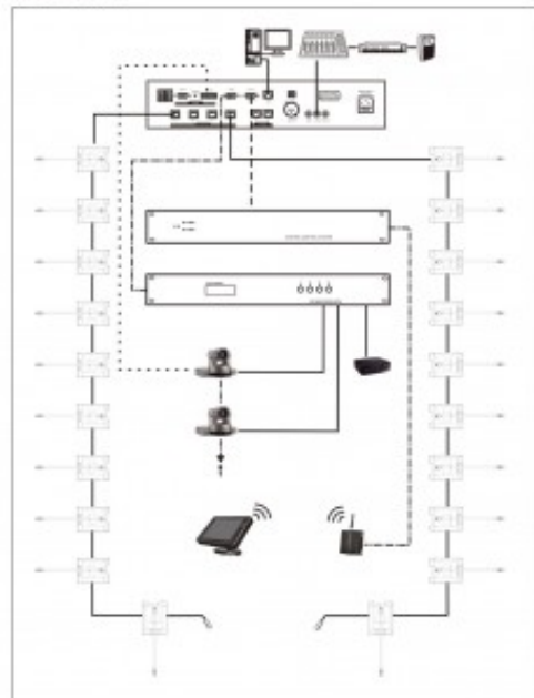
System Connection Diagram
