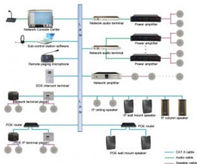
M-6000 Series IP Network PA System Connection Drawing
