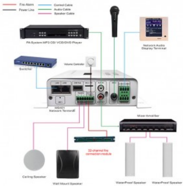
M-6401 Connection Diagram
